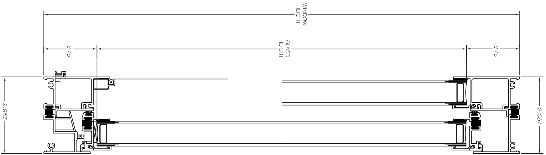
SECTION 2 SILL
